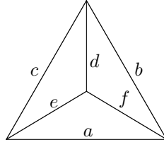
FIGURE 2. The six edges of a tetrahedron (a, b, c, d, e, f) .
