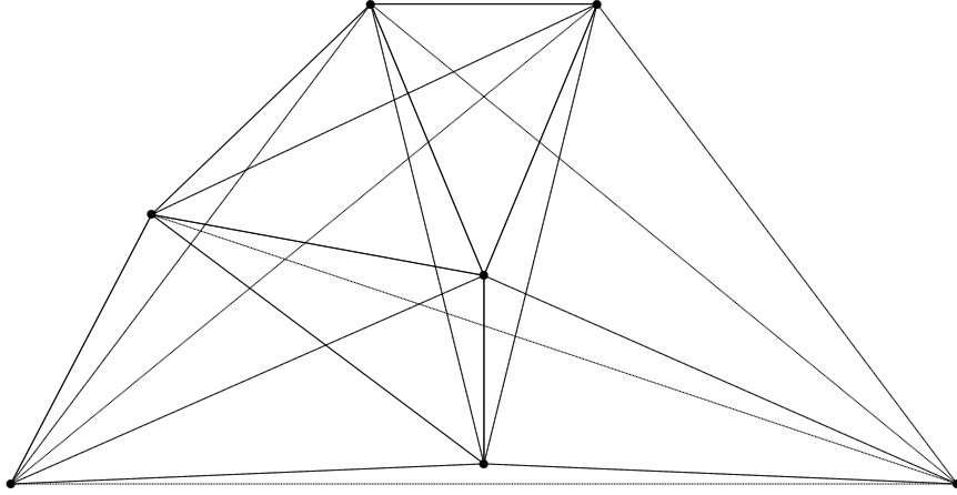
FIGURE 1. Almost a 7_2 -cluster.
