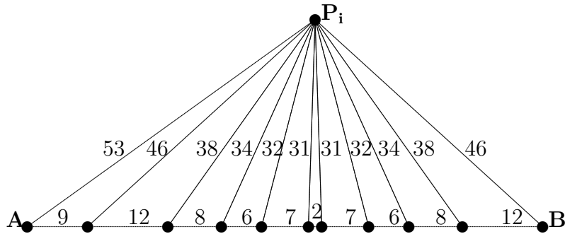
Figure 6. 2-dimensional integral point set with n = 12 and diameter 77.
