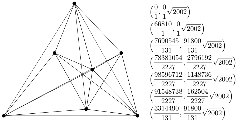
Figure 2: Second example of an integral heptagon in general position.
